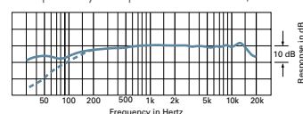
frequency response: 80–20,000 Hz
