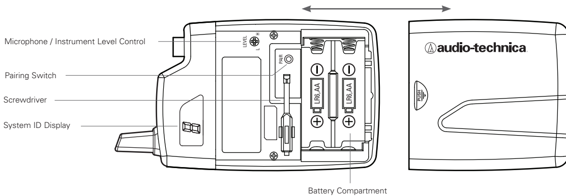
Figure C – ATW-T1001 UniPak® Transmitter
