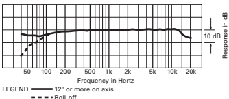
frequency response: 40–16,000 Hz
