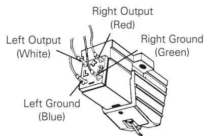
Figure 8 – Electrical Connections
