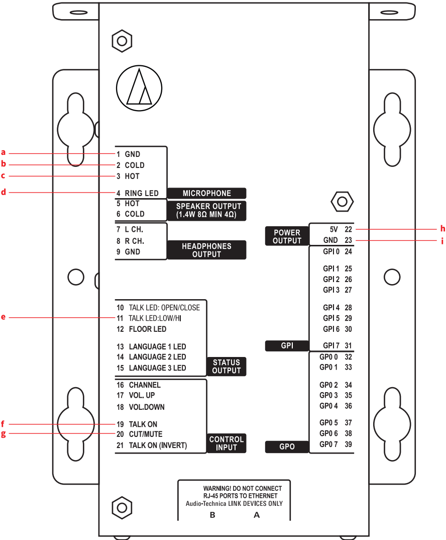
Connection Wire Specification (FM01/FM02 to ATUC-50IU) : 20AWG - 26AWG
