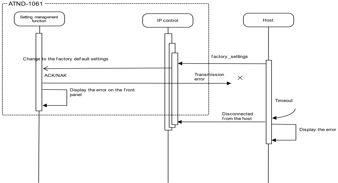
Figure 4-6 Sequence for Transmission Errors
