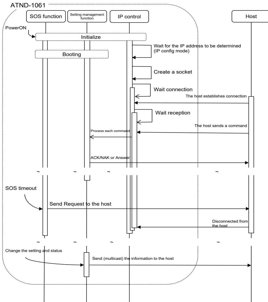
Figure 4-1 Communication Control Flow
