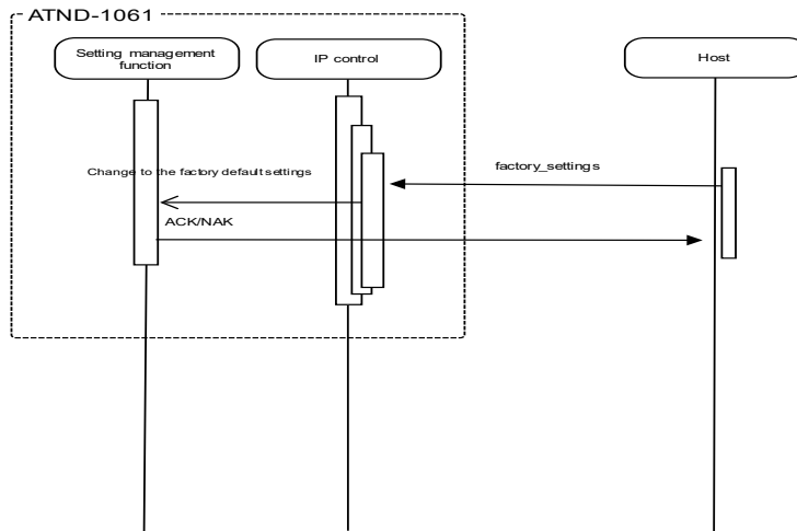
Figure 4-2 Set Command Processing Sequence
