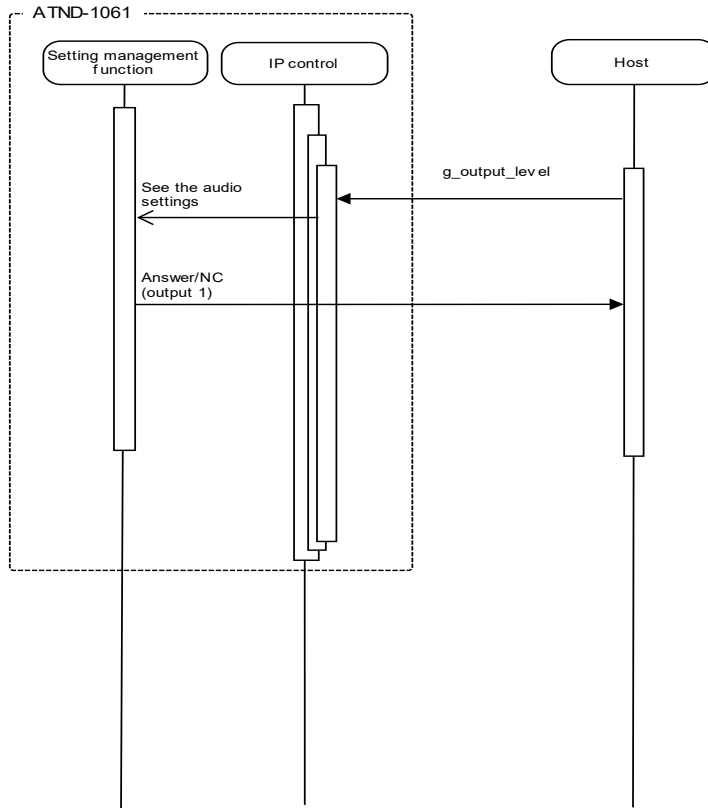
Figure 4-3 Get Command Processing Sequence
