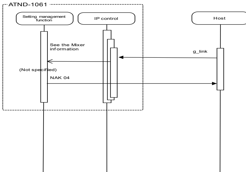
Figure 4-4 Get Command Processing Sequence (NAK)
