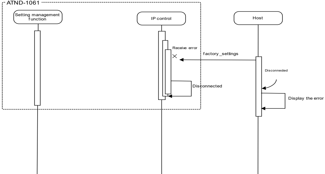
Figure 4-7 Sequence for Receive Errors
