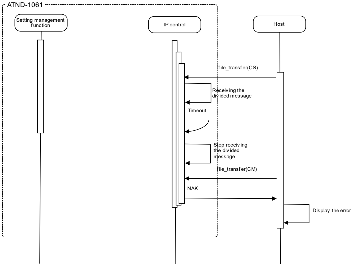
Figure 4-8 Sequence for Message Split Receive Timeouts
