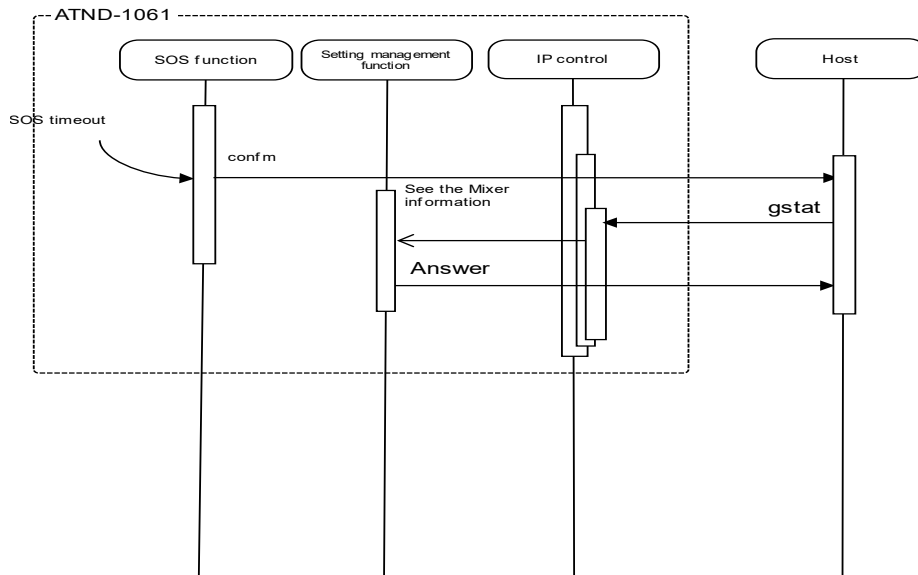
Figure 4-5 Request Command Processing Sequence
